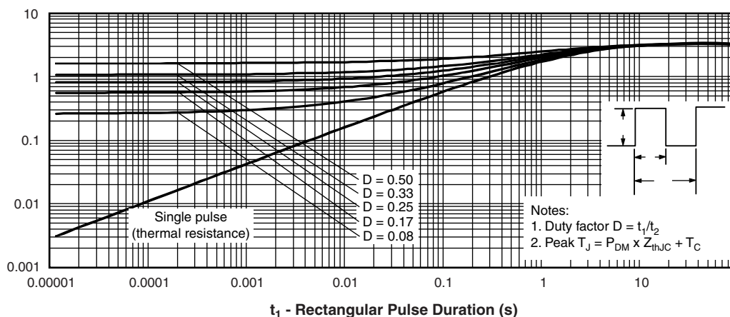
Fig. 4 - Maximum Thermal Impedance Z_{thJC} Characteristics (Per Leg)
