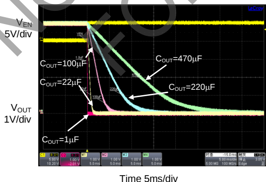
Output Turn Off and Fall Time ( V_{\text{IN}} = 5\text{V} , C_{\text{IN}} = 1.0\mu\text{F} , No Load)
