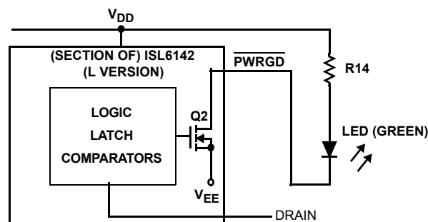
FIGURE 36. ACTIVE LOW ENABLE LED
