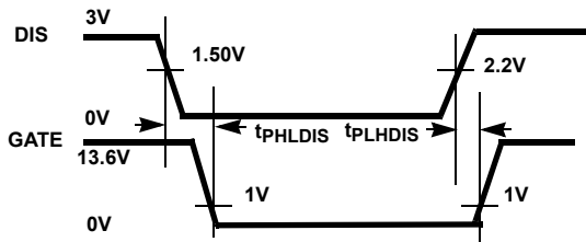
FIGURE 7. DISABLE TO GATE TIMING (ISL6142/52)
