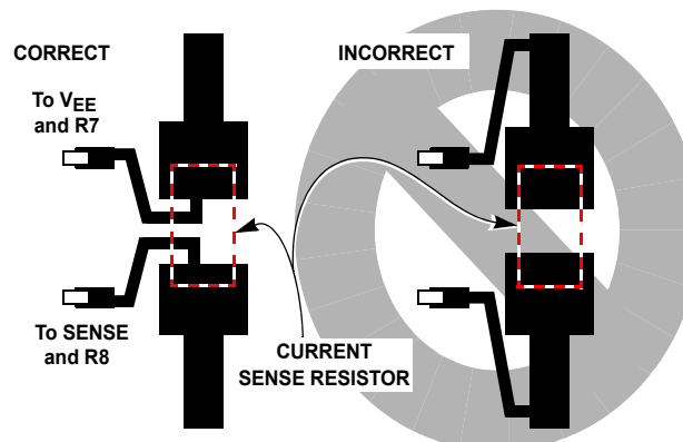
FIGURE 30. SENSE RESISTOR LAYOUT GUIDELINES
