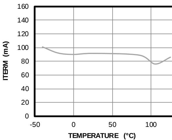
I TERM = 100mA vs. Temperature
