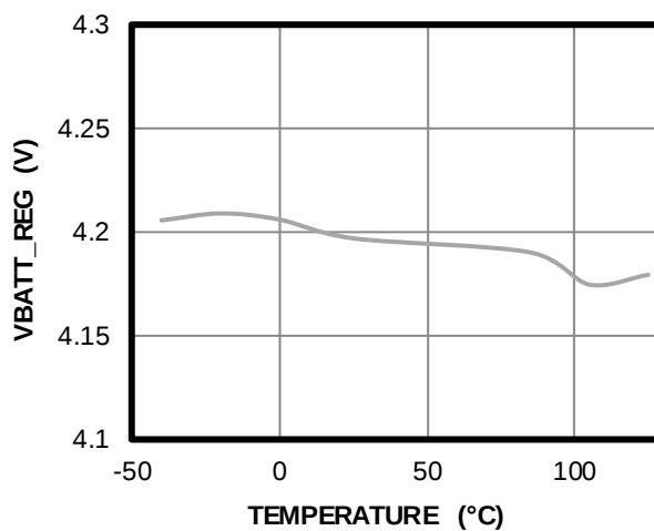
V BATT_REG = 4.2V vs. Temperature
