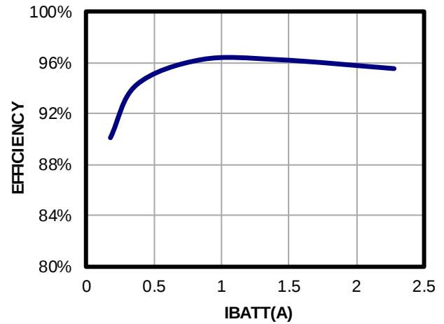
Constant Voltage Charge Efficiency
