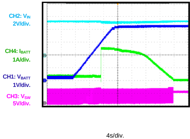
Pre-Charge Steady State
