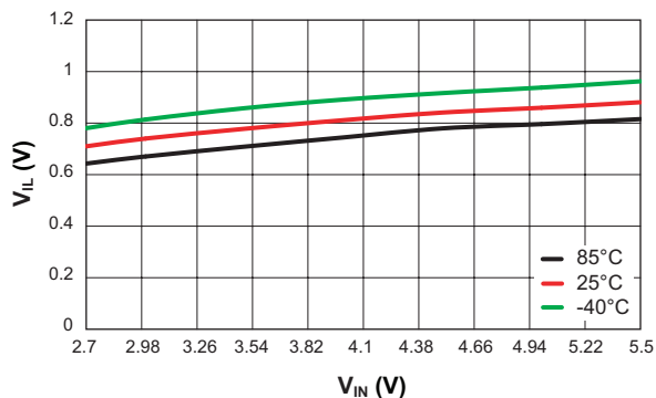
Input Low Voltage vs. Input Voltage
