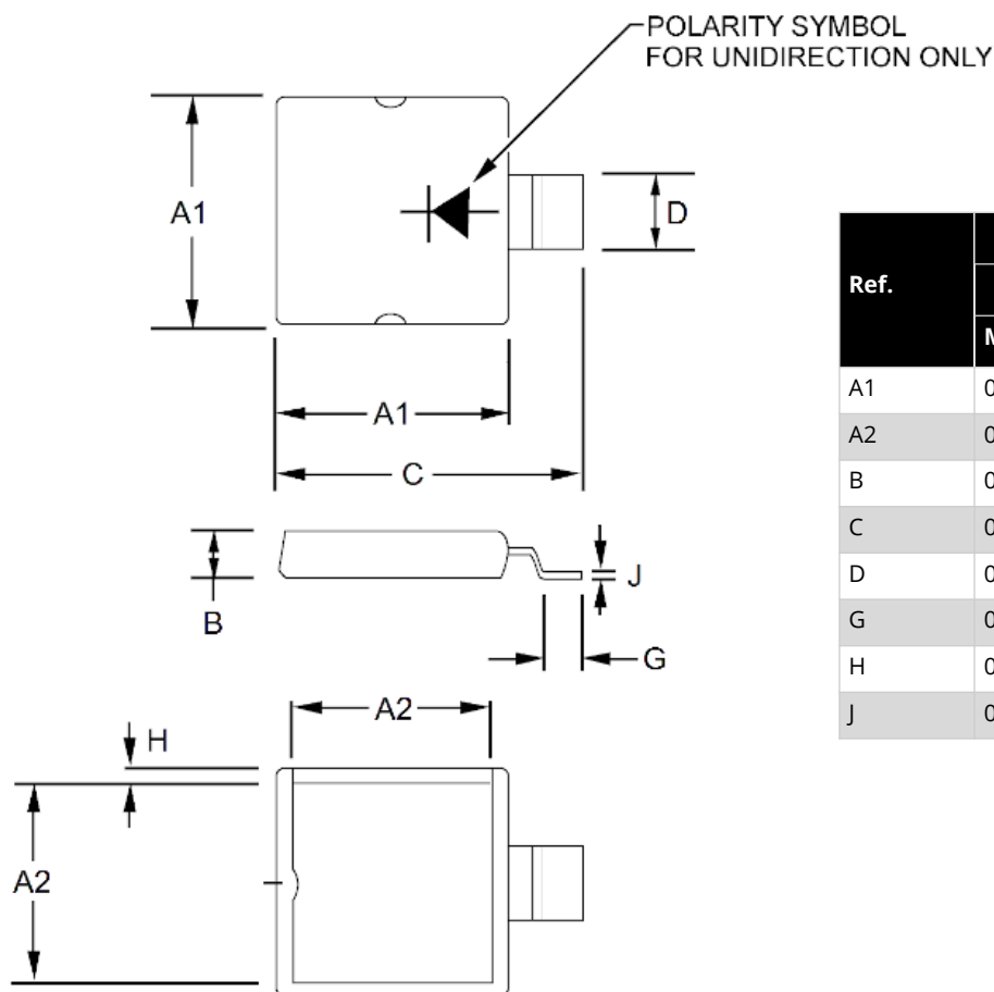
Figure 5-1. Package Dimensions
