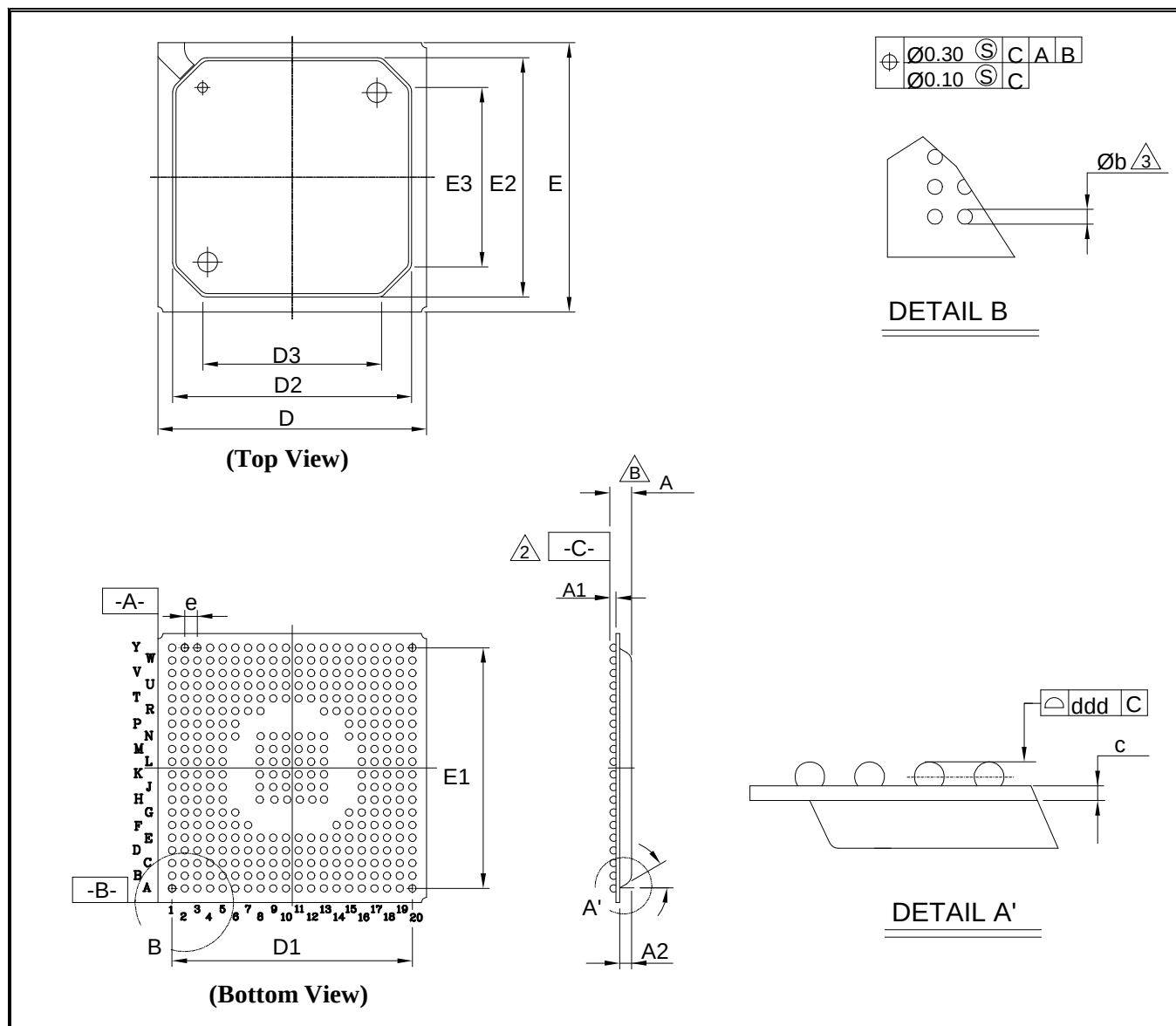
Figure 40. 352 Pin PBGA Pin Diagram
