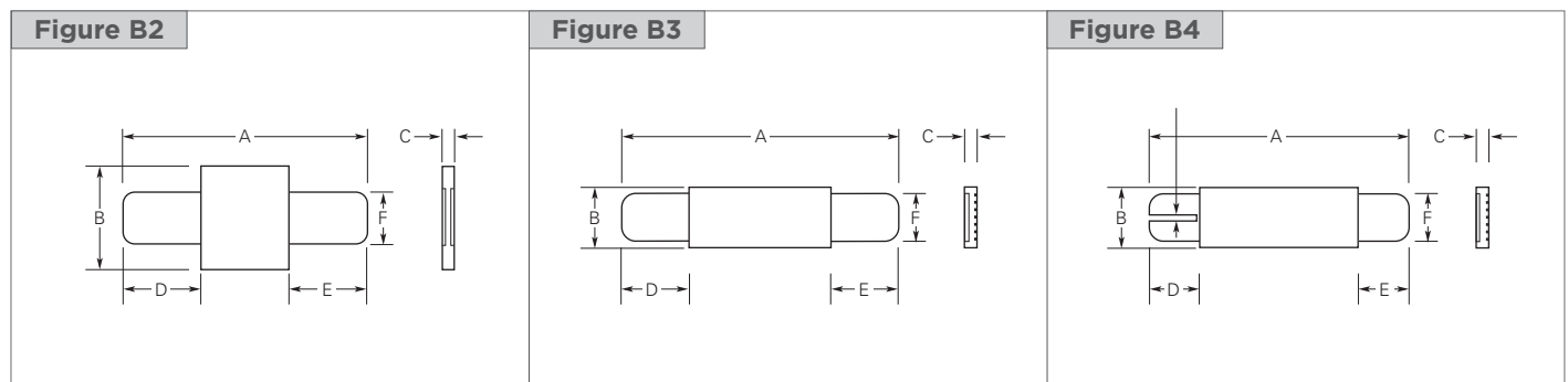
Figures B2-B12 — Dimension Figures
