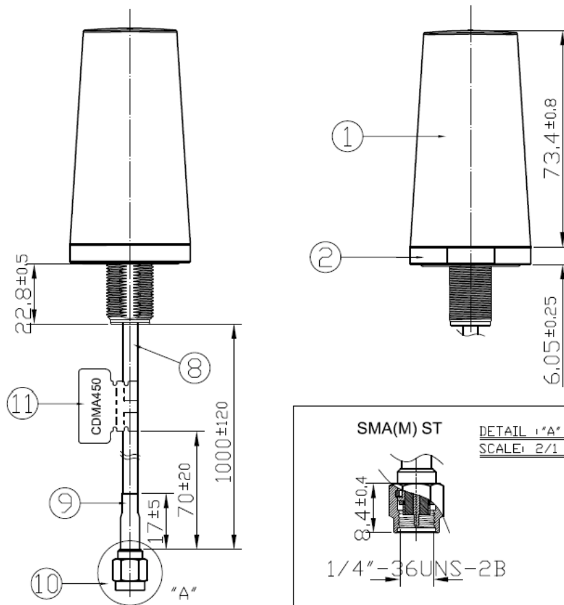
Side View
