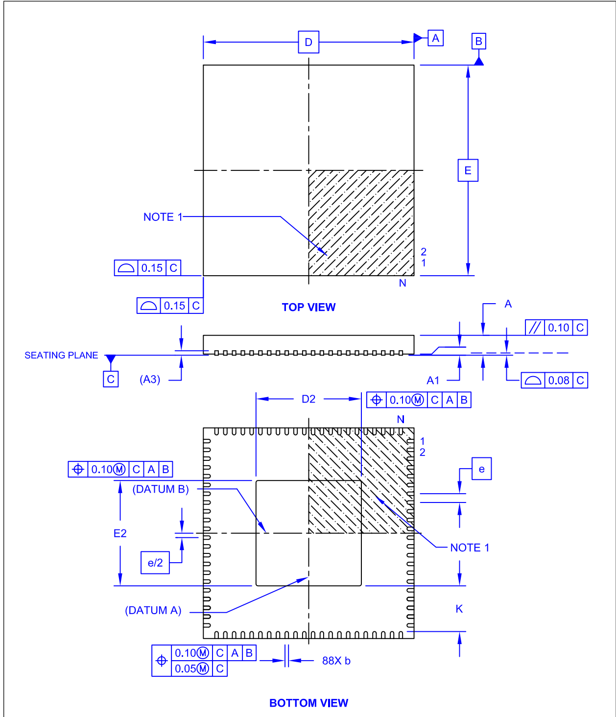
FIGURE 21-1: 88-QFN PACKAGE
