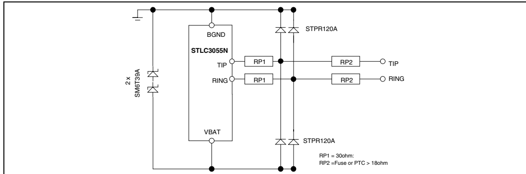
Figure 19. Simplified configuration for indoor overvoltage protection
