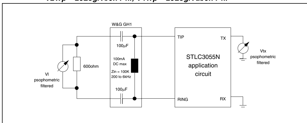
Figure 18. V2Wp and W4Wp: idle channel psophometric noise at line and TX. V2Wp = 20\text{Log}|V_I/0.774I| ; V4Wp = 20\log|V_{tx}/0.774I|
