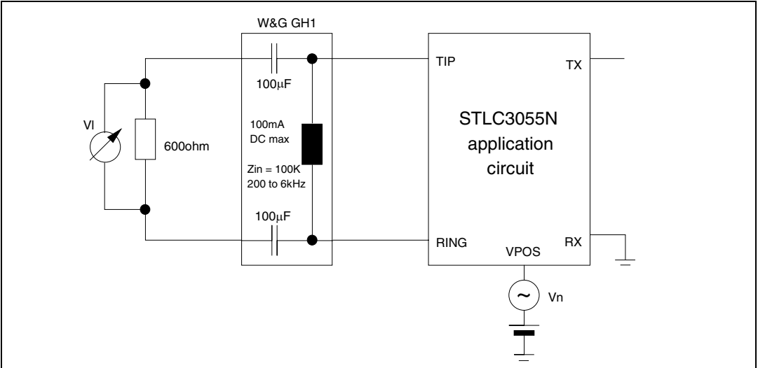
Figure 14. PSRRC power supply rejection V_{pos} to 2W port PSSRC = 20\text{Log}|V_n/V_I|
