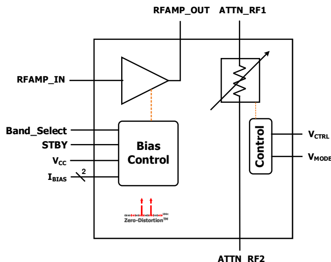
Figure 1. Block Diagram
