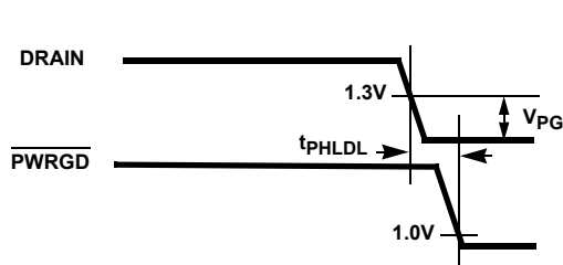
FIGURE 4A. DRAIN TO \overline{\text{PWRGD}} ACTIVE TIMING (ISL6142)
