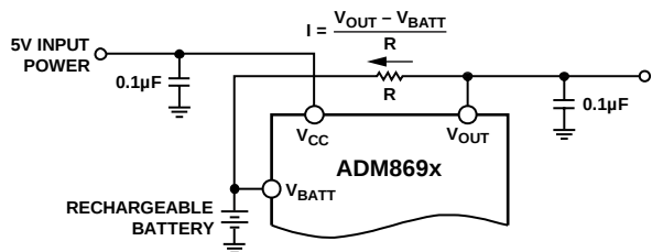
Figure 25. Rechargeable Battery
