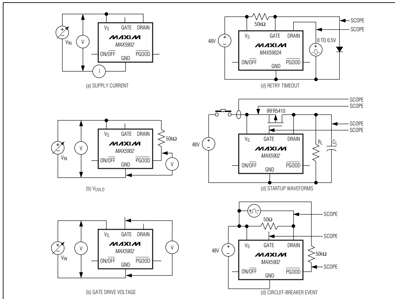
Figure 2. Test Circuits
