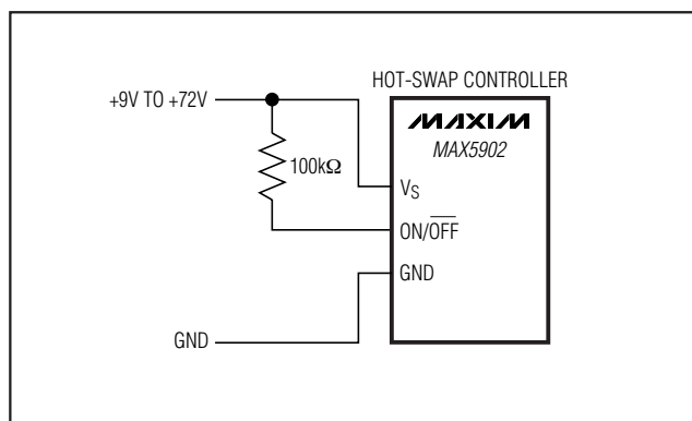
Figure 6. Defeating Undervoltage Lockout
