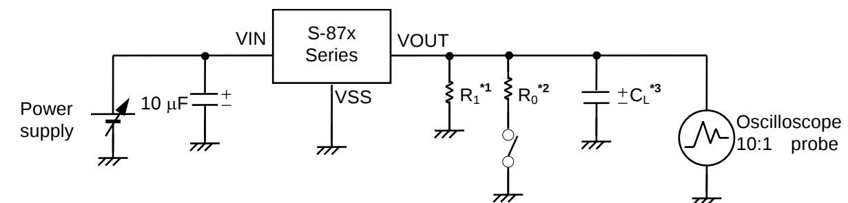
Figure 31 Output voltage fluctuation due to a change in the load current
