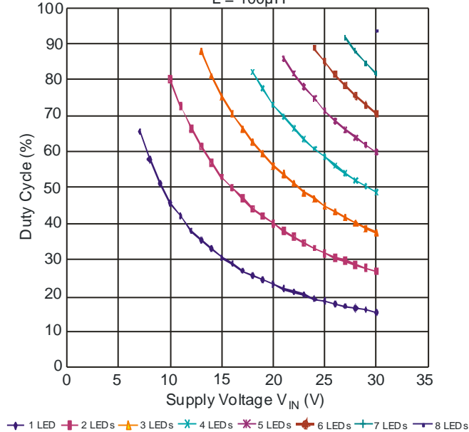
ZXLD1360 Duty Cycle L = 100\mu\text{H}
