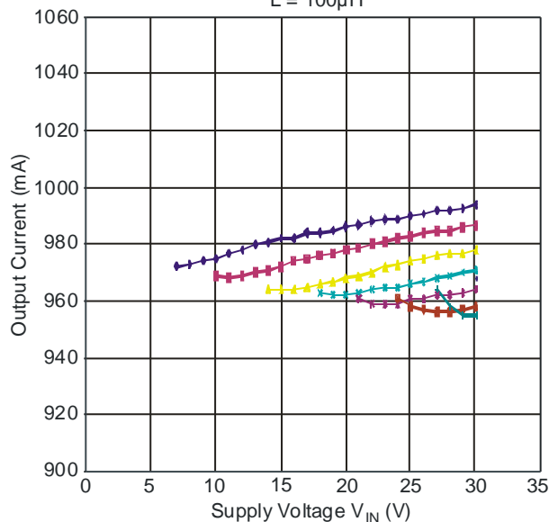
ZXLD1360 Output Current L = 100\mu\text{H}
