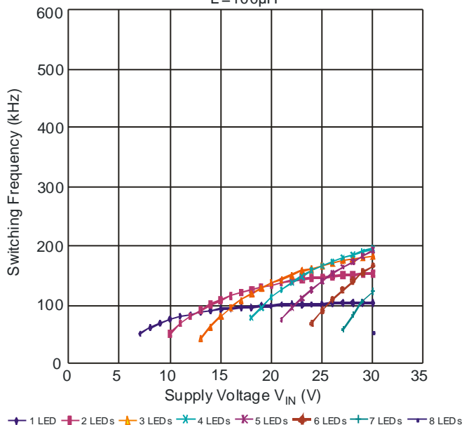
ZXLD1360 Switching Frequency L = 100\mu\text{H}
