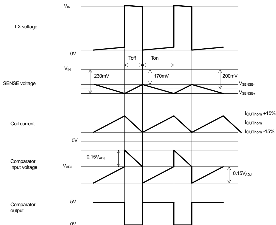
Figure 2 Operating Waveforms
