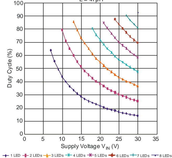
ZXLD1360 Duty Cycle L = 47\mu\text{H}
