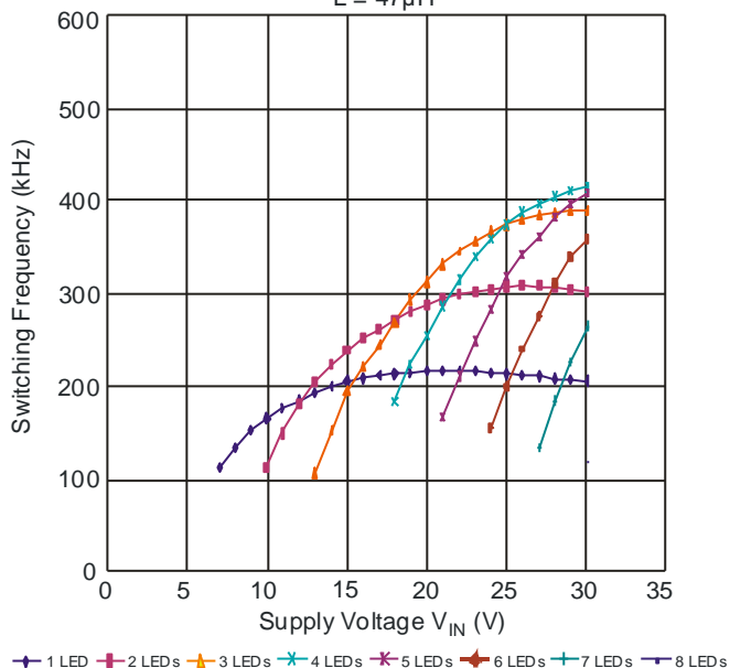
ZXLD1360 Switching Frequency L = 47\mu\text{H}
