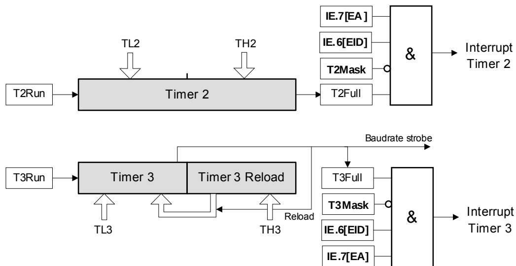
Figure 50 Timer 2/3 - Mode 1
