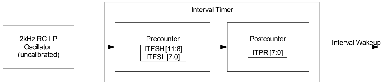
Figure 7 Interval Timer Block Diagram
