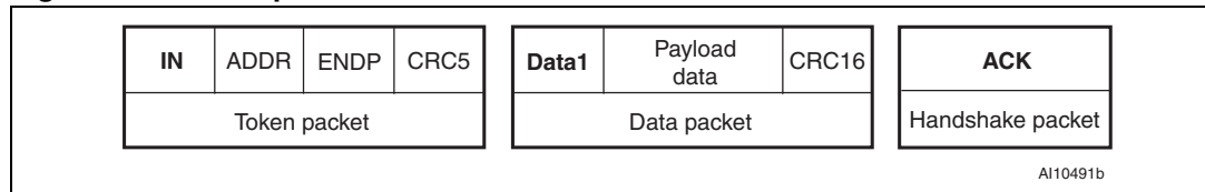
Figure 51. Interrupt transfer
