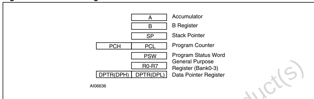
Figure 10. 8032 MCU registers
