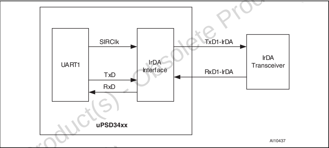
Figure 38. IrDA interface
