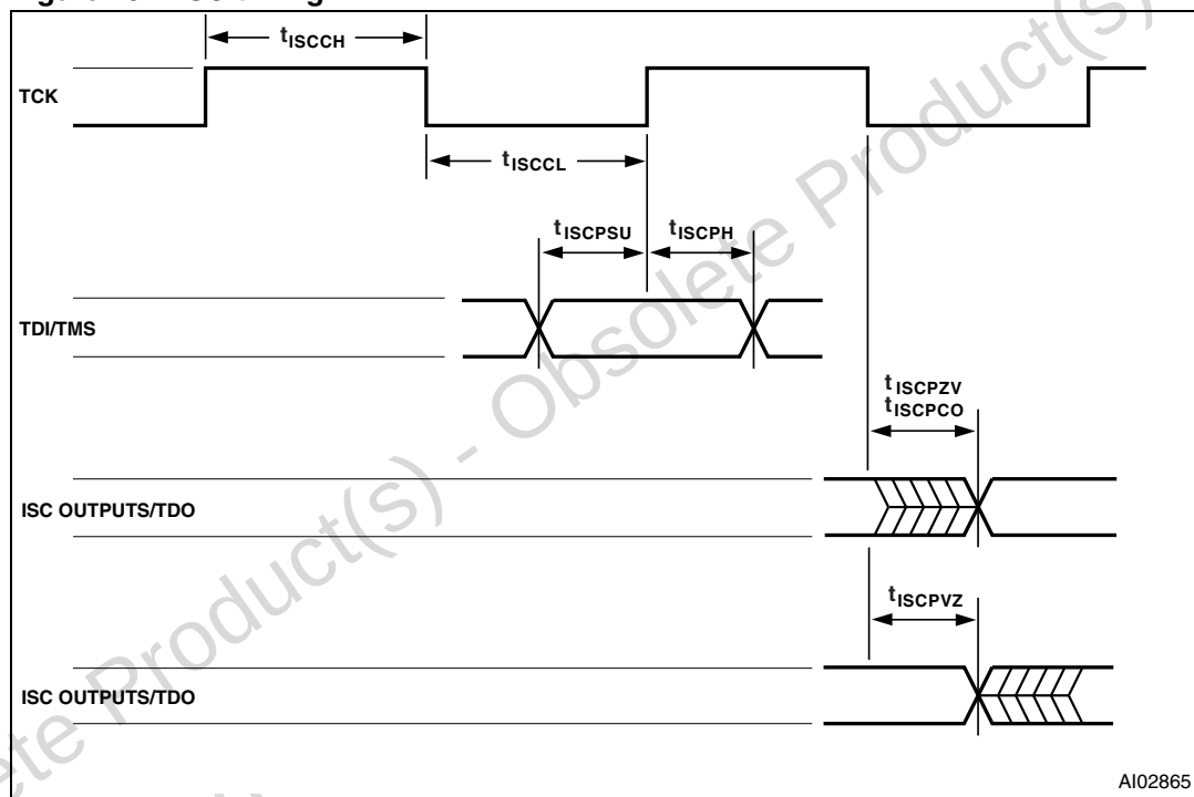
Figure 107. ISC timing
