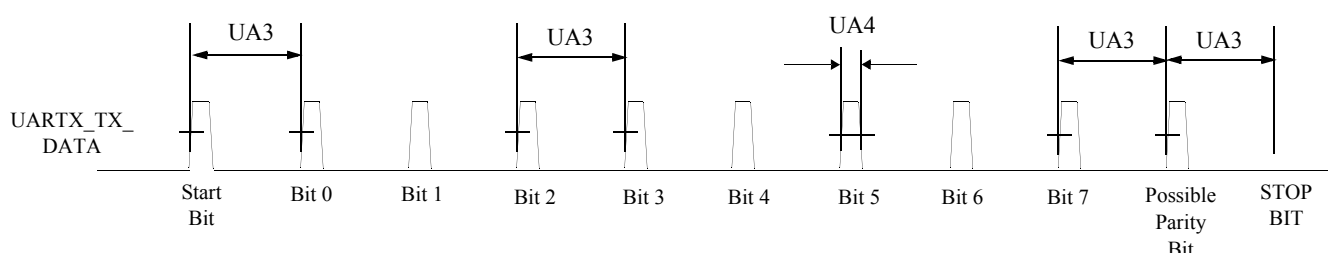
Figure 65. UART IrDA Mode Transmit Timing Diagram
