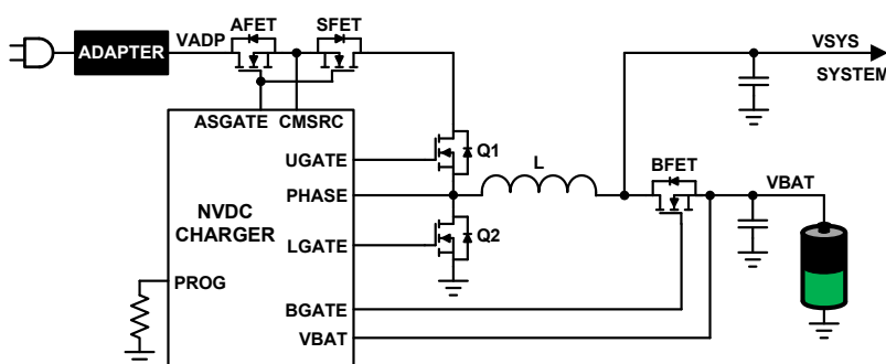
FIGURE 1. TYPICAL CONFIGURATION
