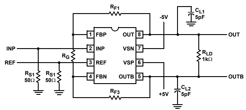
FIGURE 1. EL5171
