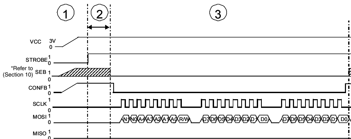
Figure 24. Startup sequence
