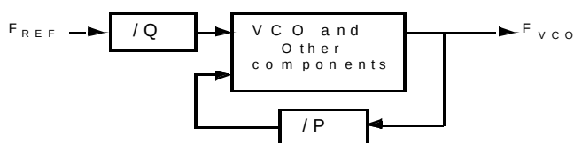
Figure 4. PLL system
