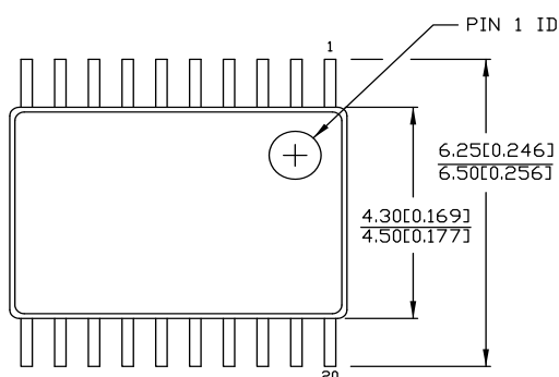
Figure 11. 20-pin TSSOP (4.40 mm Body) Z20.173/ZZ20.173 Package Outline, 51-85118
