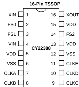
Figure 1. 16-pin TSSOP pinout
