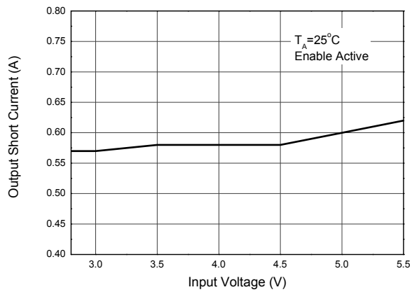
Figure 8. Output Short Current vs. Input Voltage
