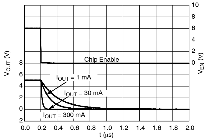
Figure 40. Shutdown, 5.0 V Version D, V_{IN} = 6.0 V
