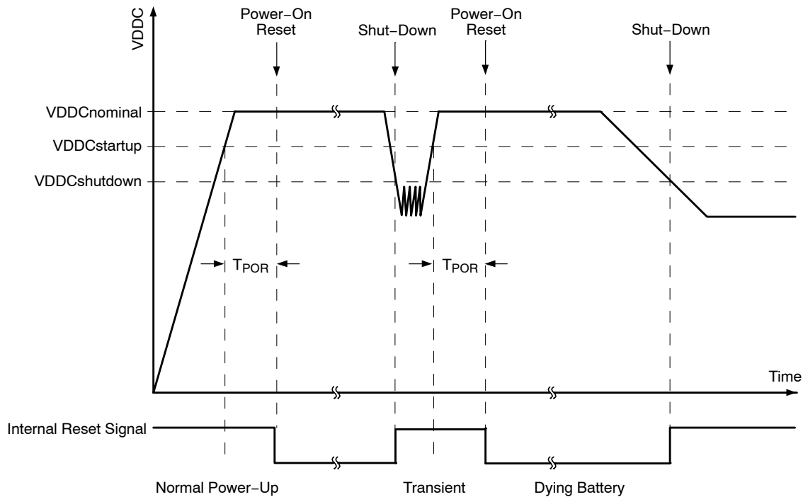
Figure 10. Power Management
