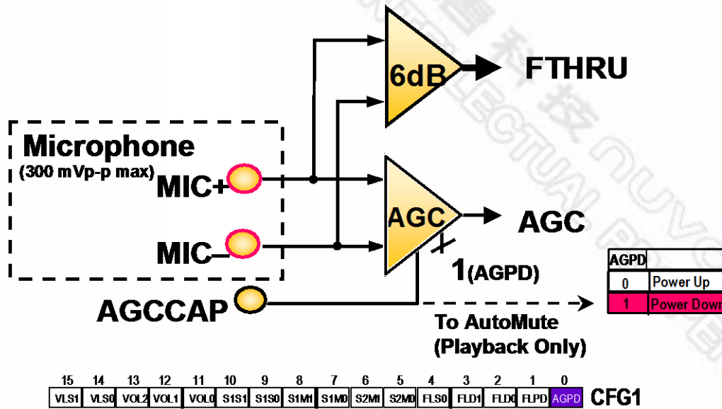
FIGURE 7: MICROPHONE AMPLIFIER
