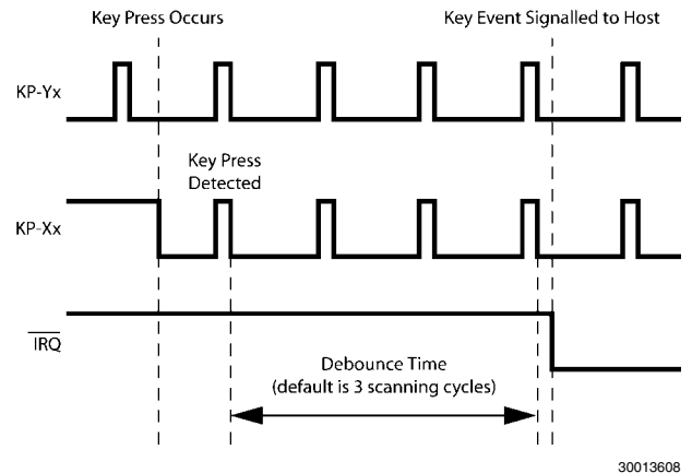
FIGURE 8. Keypad Scan Cycles
