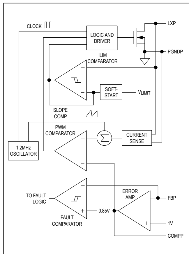
Figure 2. Boost Converter Functional Diagram
