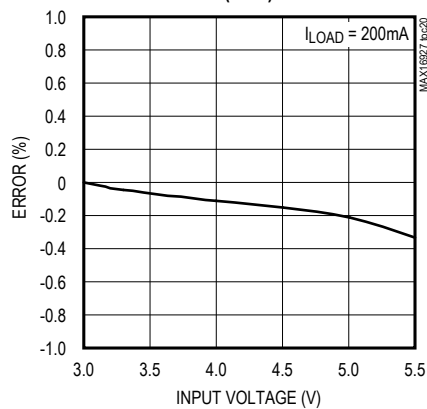
LINE REGULATION (CUK)
