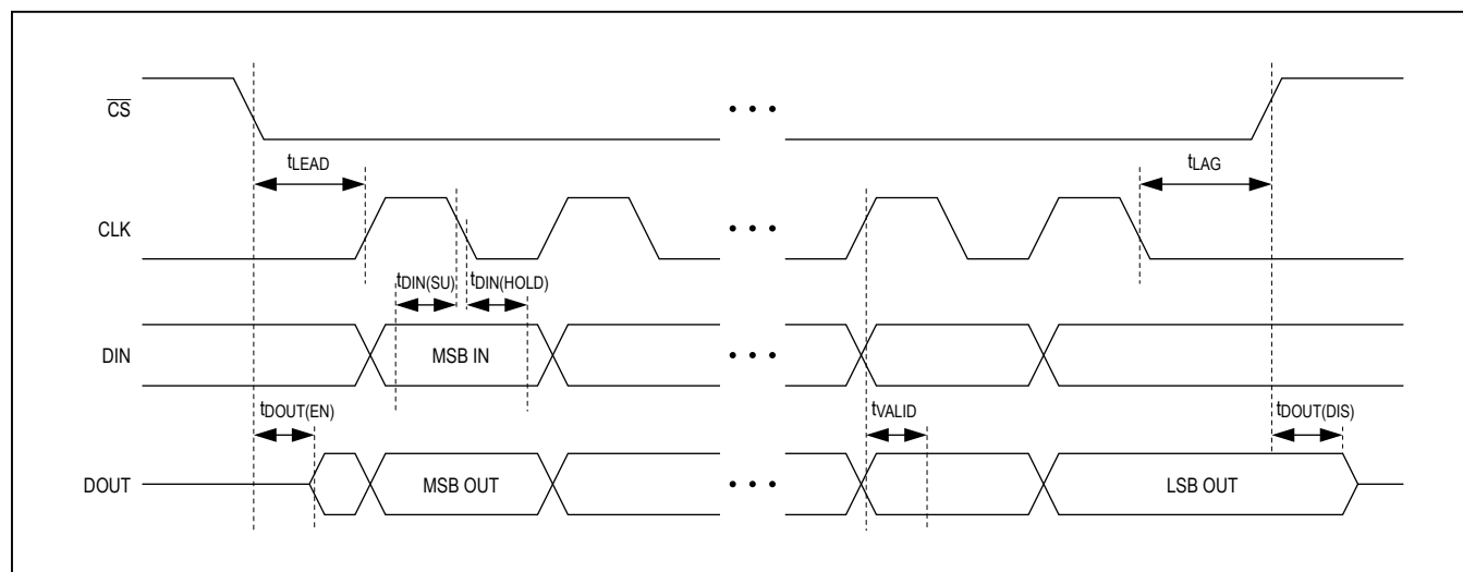
Figure 1. SPI Timing Characteristics
