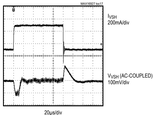
100mA TO 500mA LOAD TRANSIENT RESPONSE
