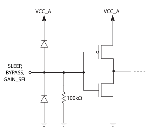
Figure 3-4: SLEEP, BYPASS, and GAIN_SEL Circuits
