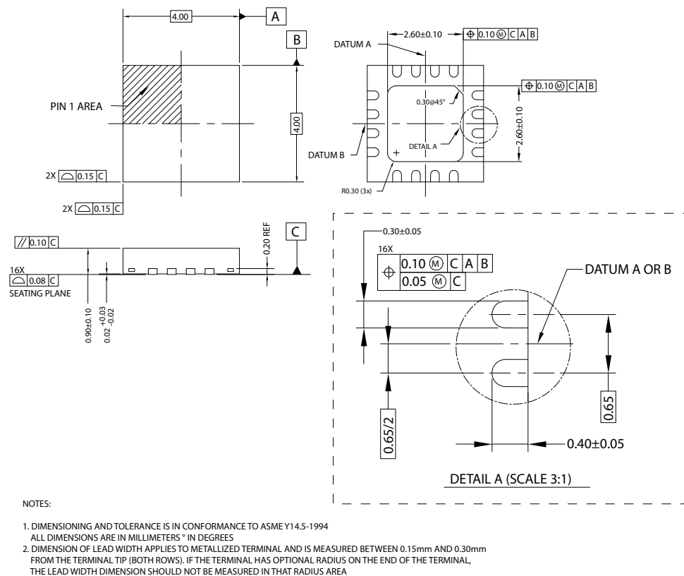
Figure 6-1: Package Dimensions
