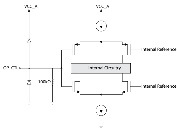
Figure 3-6: OP_CTL
