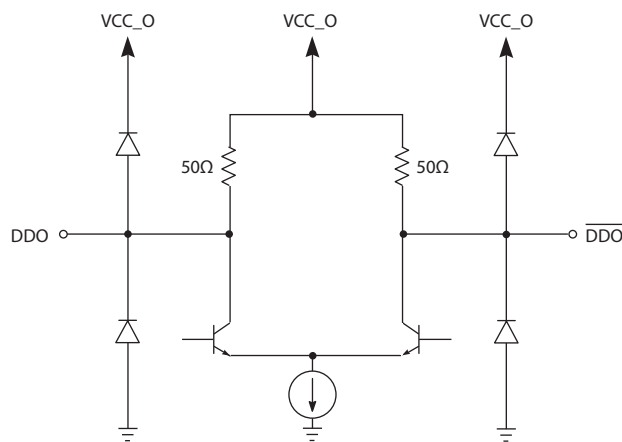
Figure 3-3: Output Circuit
