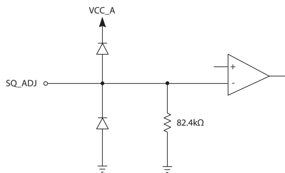
Figure 3-2: SQ_ADJ Circuit
