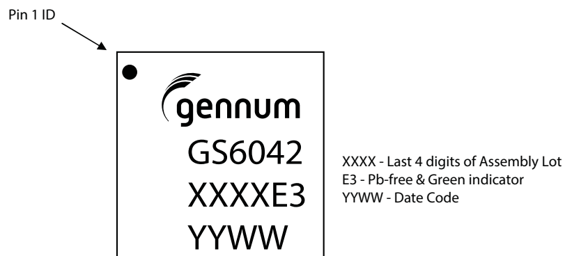
Figure 6-3: Marking Diagram
