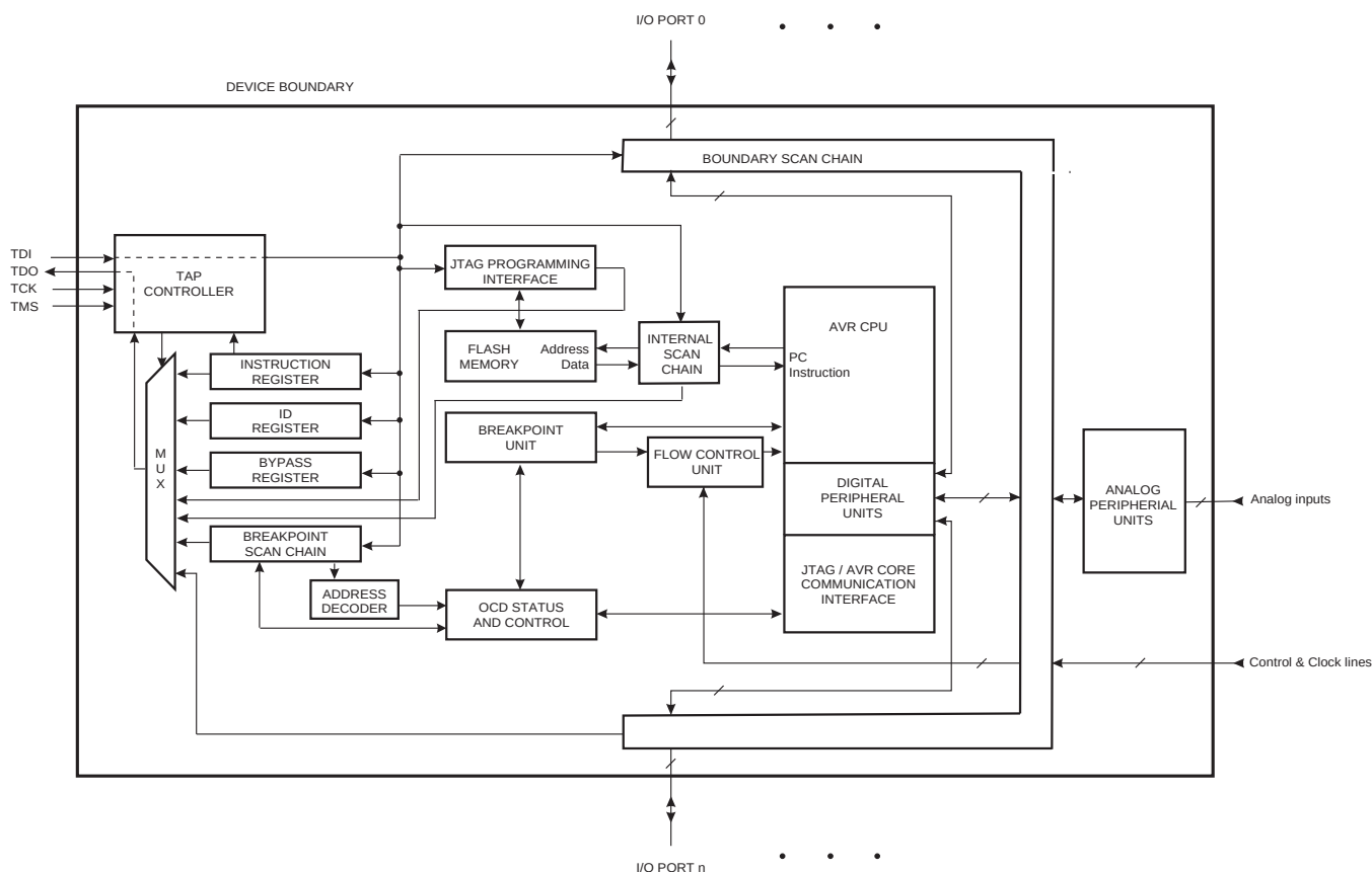
Figure 25-1. Block Diagram
