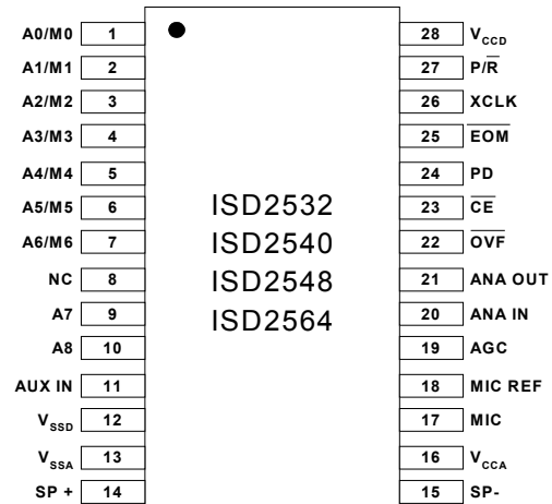
SOIC/PDIP
