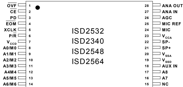
TSOP
