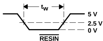
Figure 2. Input Pulse Definition
