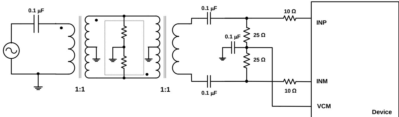
Figure 177. Driving Circuit for High Input Frequencies ( f_{IN} > 230 MHz)
