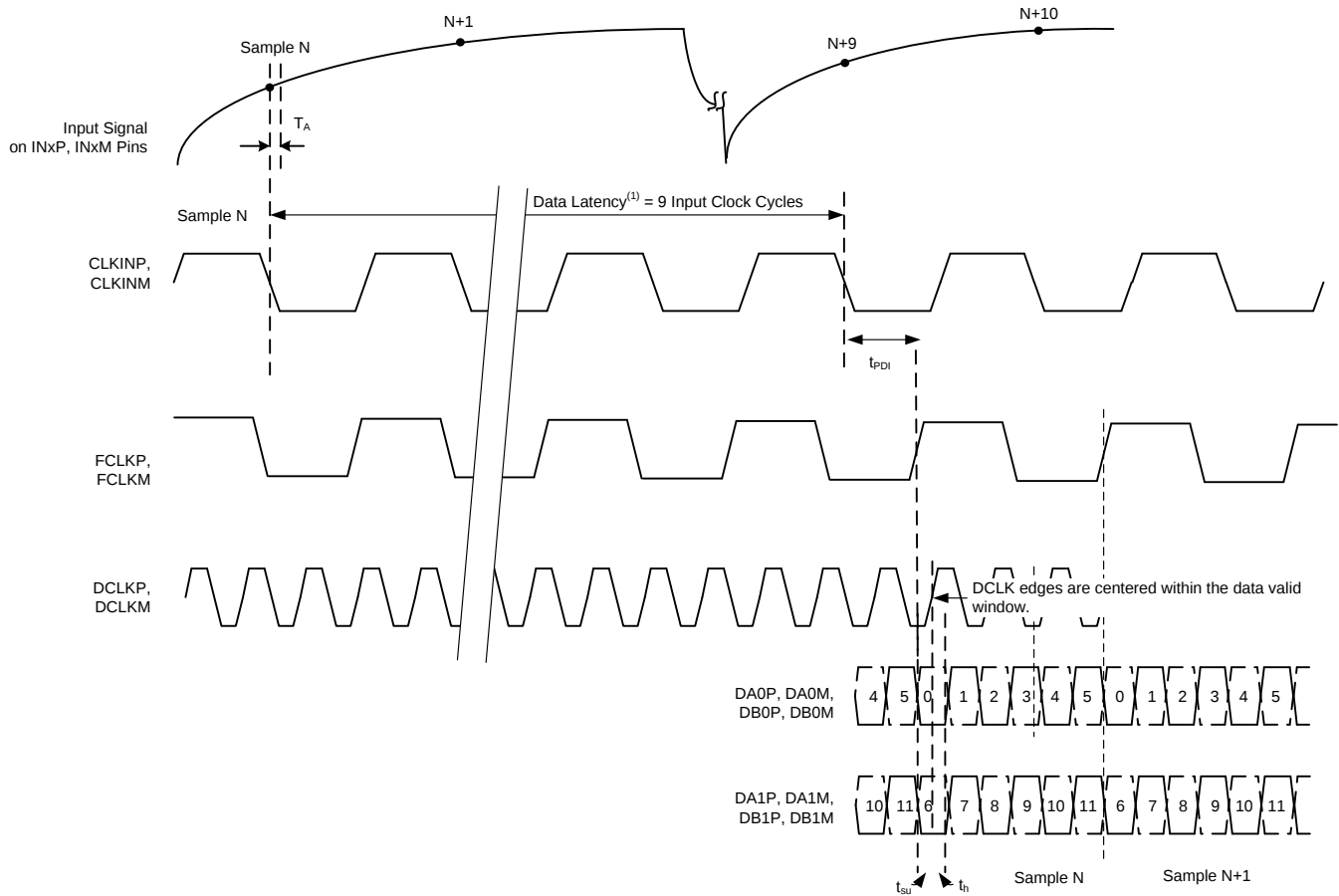
Figure 131. Latency Diagram
