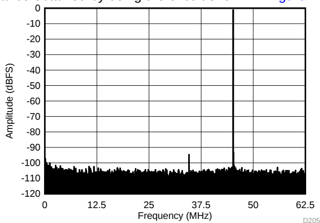
Figure 176. Performance FFT at 170 MHz (Mid Input Frequency)
