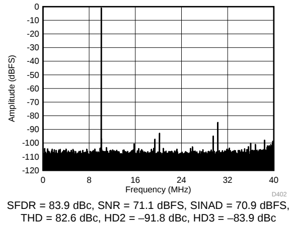
Figure 62. FFT for 10-MHz Input Signal (Dither Off)
