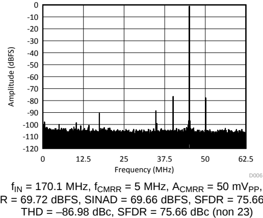
Figure 122. Common-Mode Rejection Ratio Spectrum
