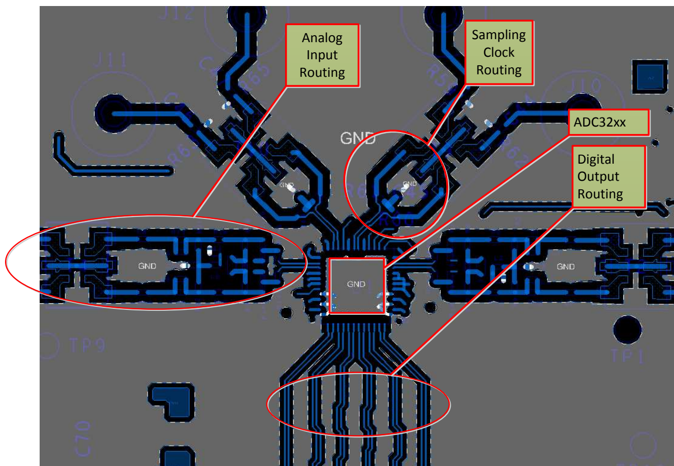
Figure 179. Typical Layout of the ADC322x Board
