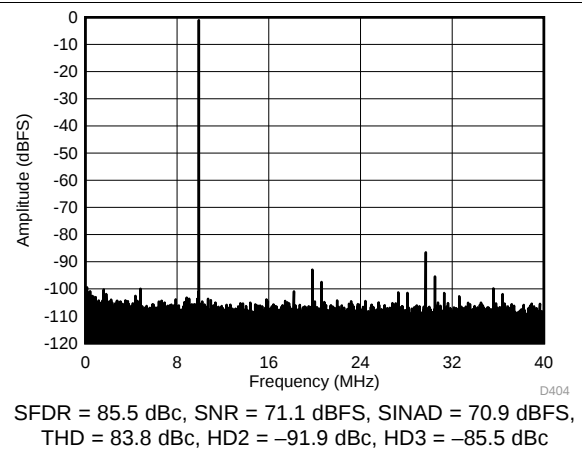
Figure 64. FFT for 70-MHz Input Signal (Dither Off)
