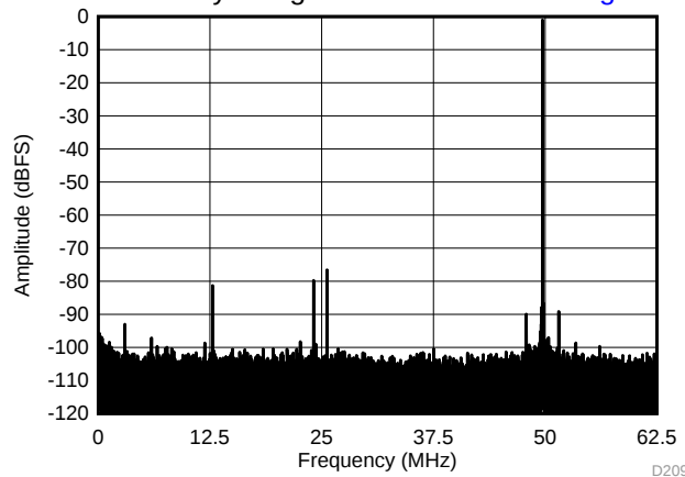
Figure 178. Performance FFT at 450 MHz (High Input Frequency)
