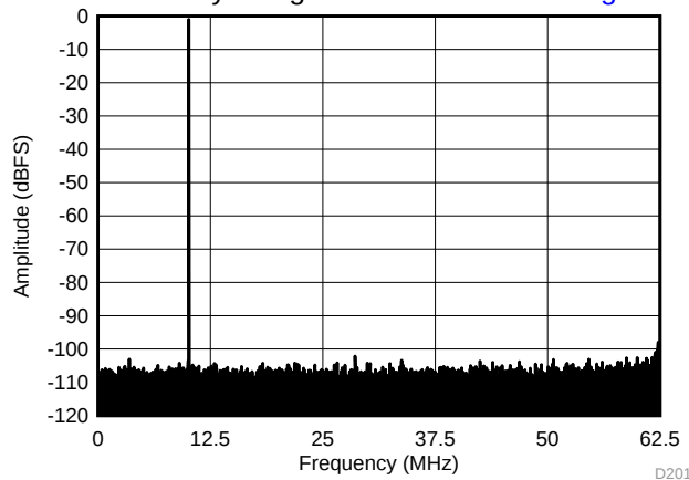
Figure 174. Performance FFT at 10 MHz (Low Input Frequency)
