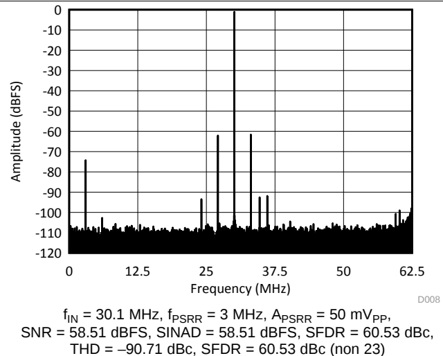
Figure 124. Power-Supply Rejection Ratio Spectrum
