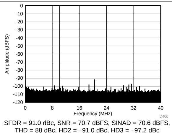
Figure 66. FFT for 170-MHz Input Signal (Dither Off)
