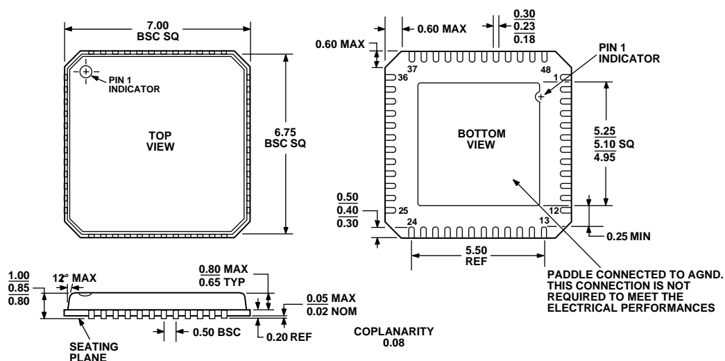
Figure 47. 48-Lead Frame Chip Scale Package (LFCSFP) [CP-48] Dimensions shown in millimeters
