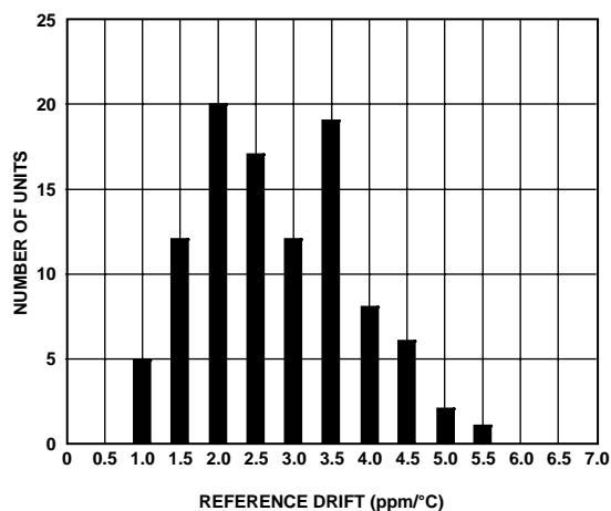
Figure 22. Reference Voltage Temperature Coefficient Distribution (102 Units)
