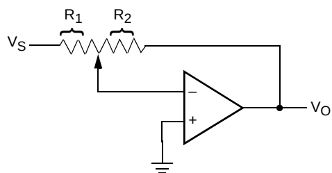
INVERTING AMPLIFIER
