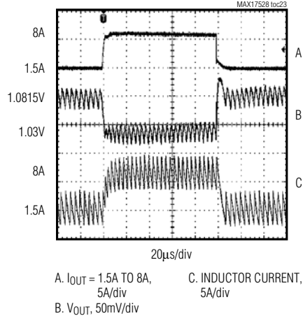
LOAD-TRANSIENT RESPONSE
