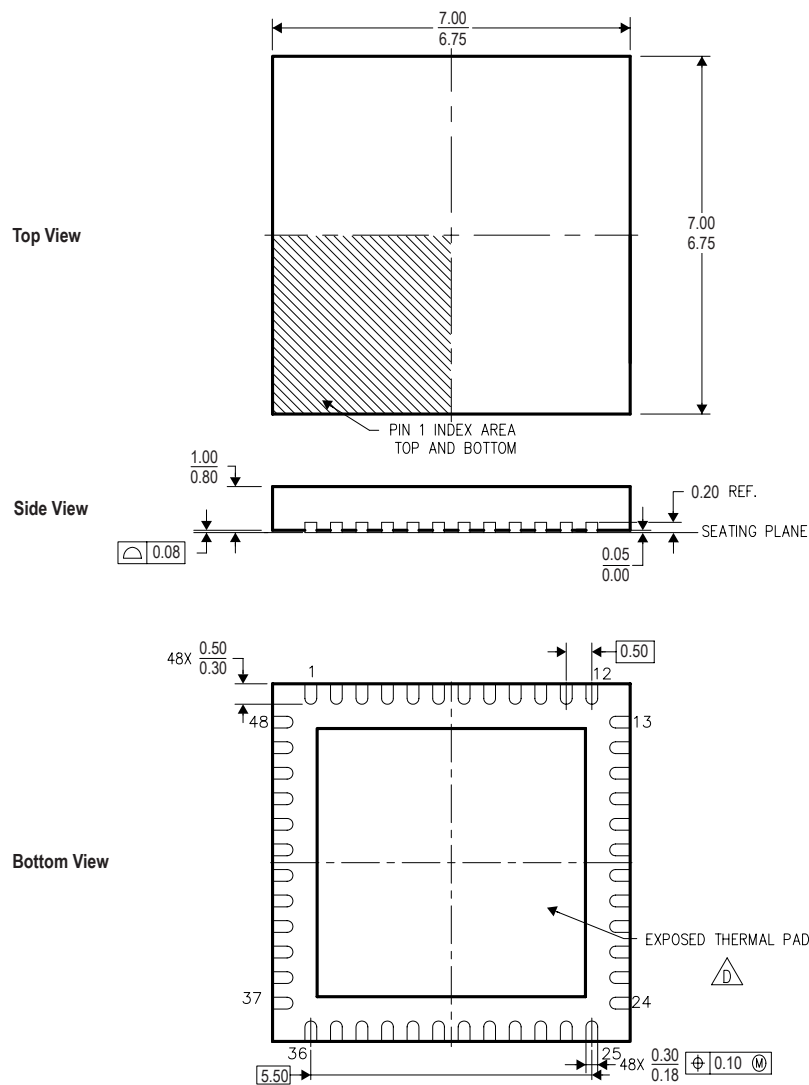
Figure D-4. Stellaris LM3S815 48-Pin QFN Package
