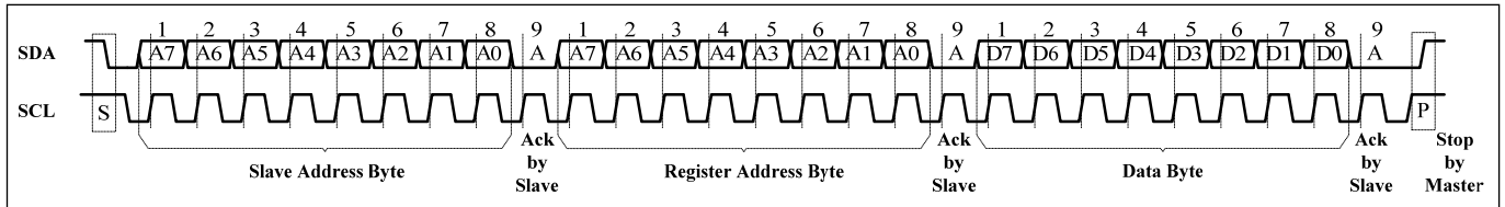
Figure 5 Writing to IS31FL3197 (Typical)
