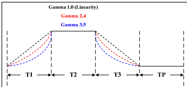
Figure 11 Gamma Correction
