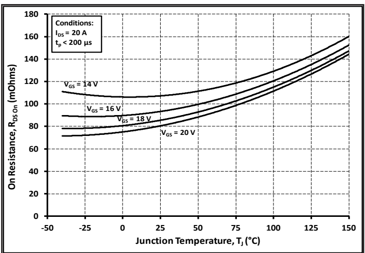
Figure 6. On-Resistance vs. Temperature for Various Various Gate-Source Voltages
