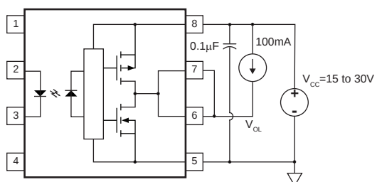
V_{OL} Test Circuit
