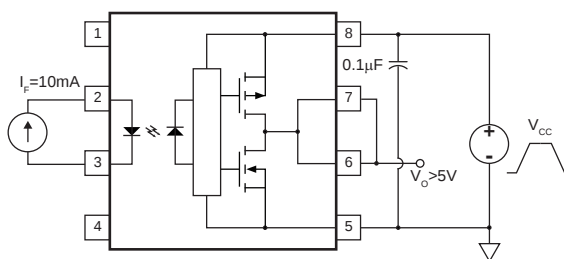
UVLO Test Circuit
