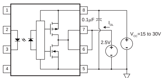
I_{OL} Test Circuit
