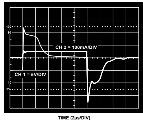
Figure 33. Scope Photo of the V_{COM} Instantaneous Peak Current
