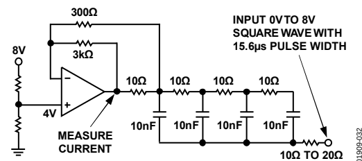
Figure 32. V_{COM} Test Circuit with Supply Voltage at 16 V
