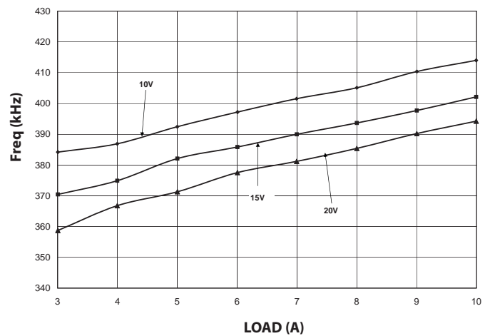
Frequency vs. Load, VOUT2 at 1.5V
