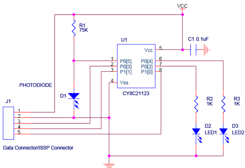
Figure A-6. Demo Board Schematic
