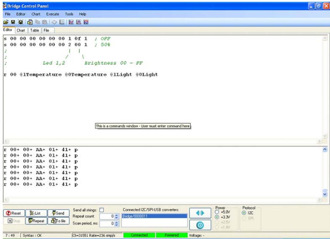
Figure 3-8. Bridge Control Panel Editor Screen View
