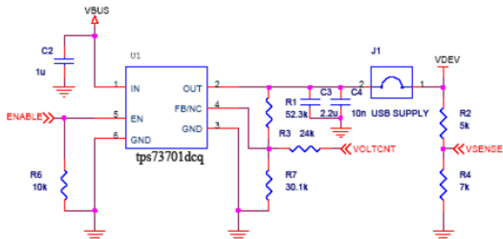
Figure A-1. Reverse Current Protection Schematic
