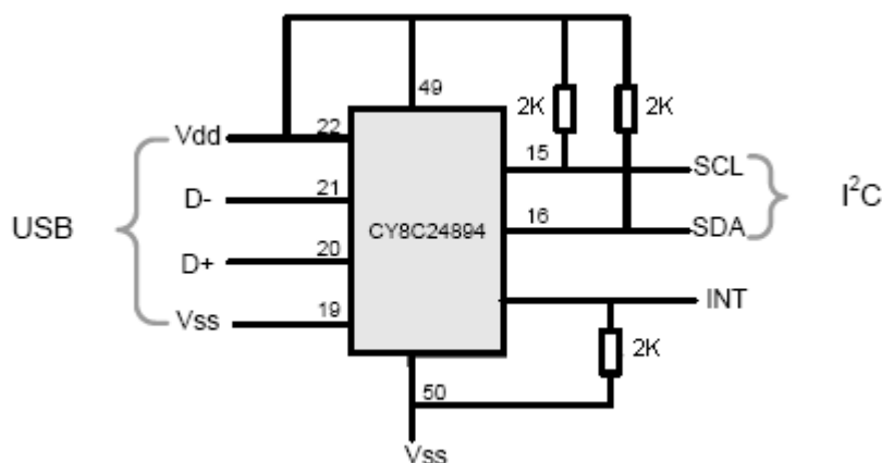
Figure 3-2. Bridge to Device Connection
