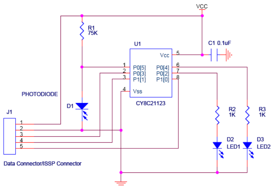
Figure 4-9. Demo Board Chip Schematic
