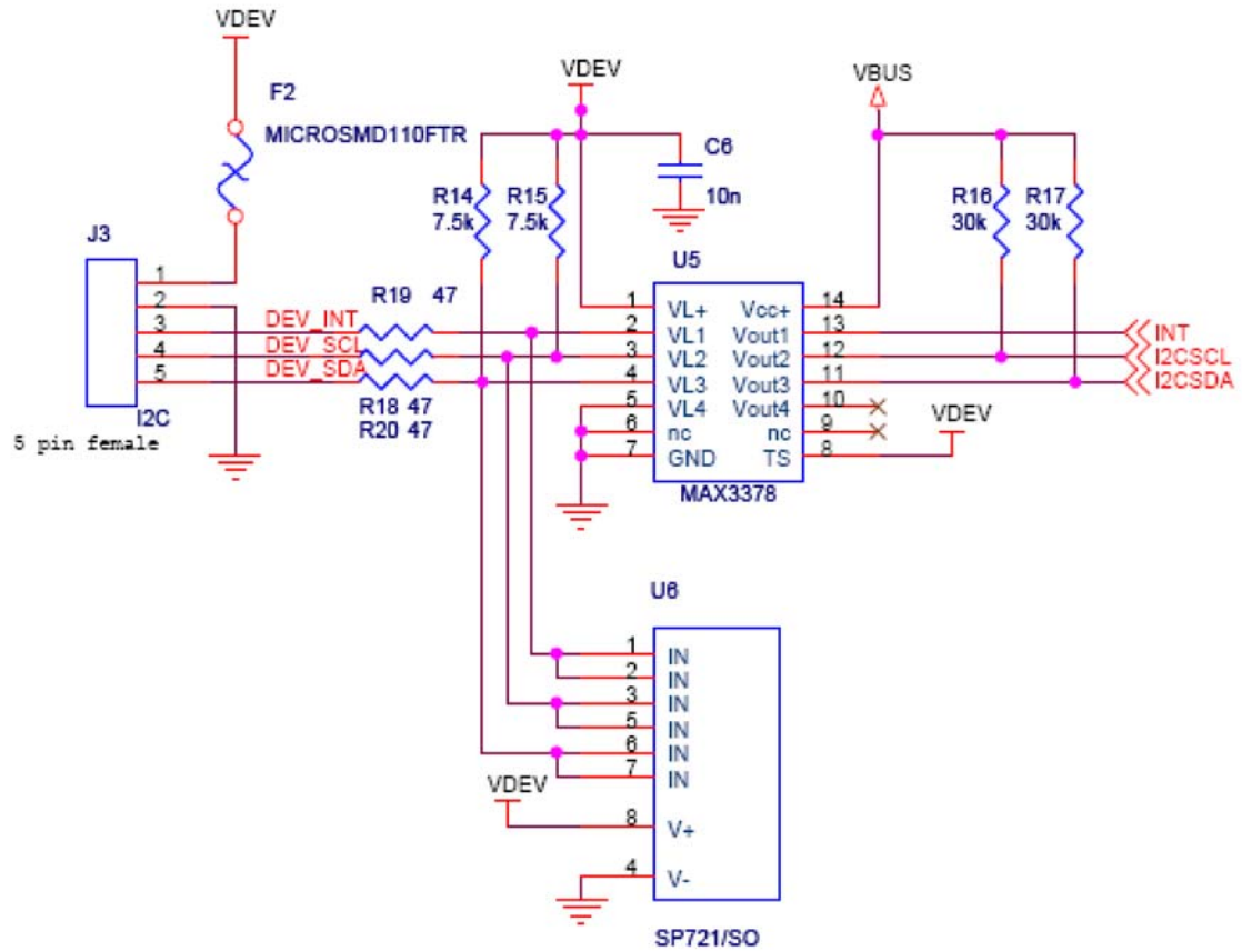
Figure 4-8. I2C Slave Interface Schematic
