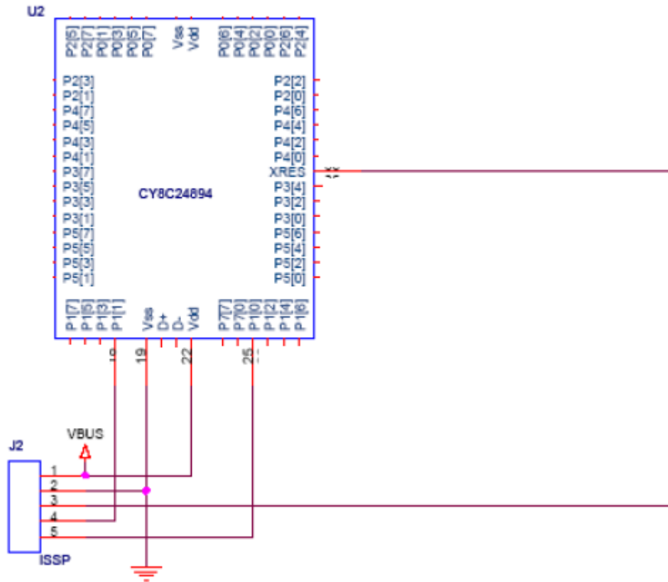
Figure 4-6. ISSP Programming Header Schematic
