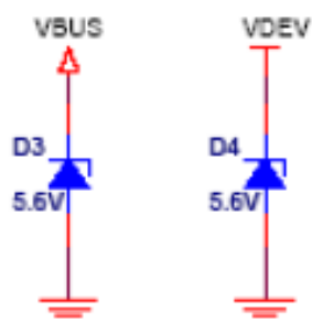
Figure A-3. Diode Schematic
