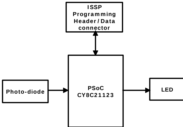
Figure 4-2. Demo Target Board
