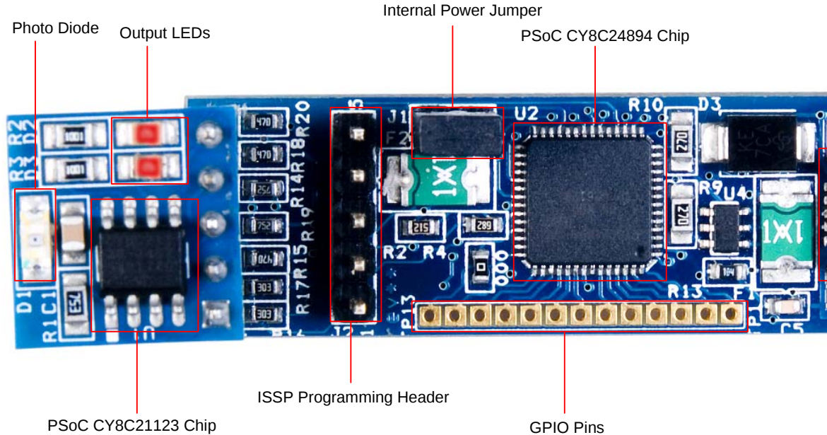
Figure 4-3. I2C-USB Bridge with Demo Target Board
