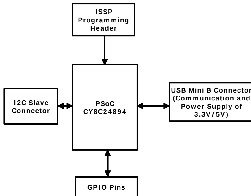
Figure 4-1. I2C-USB Bridge Board
