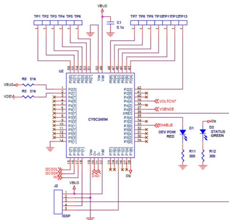
Figure A-5. PSoC CY8C24894 Schematic
