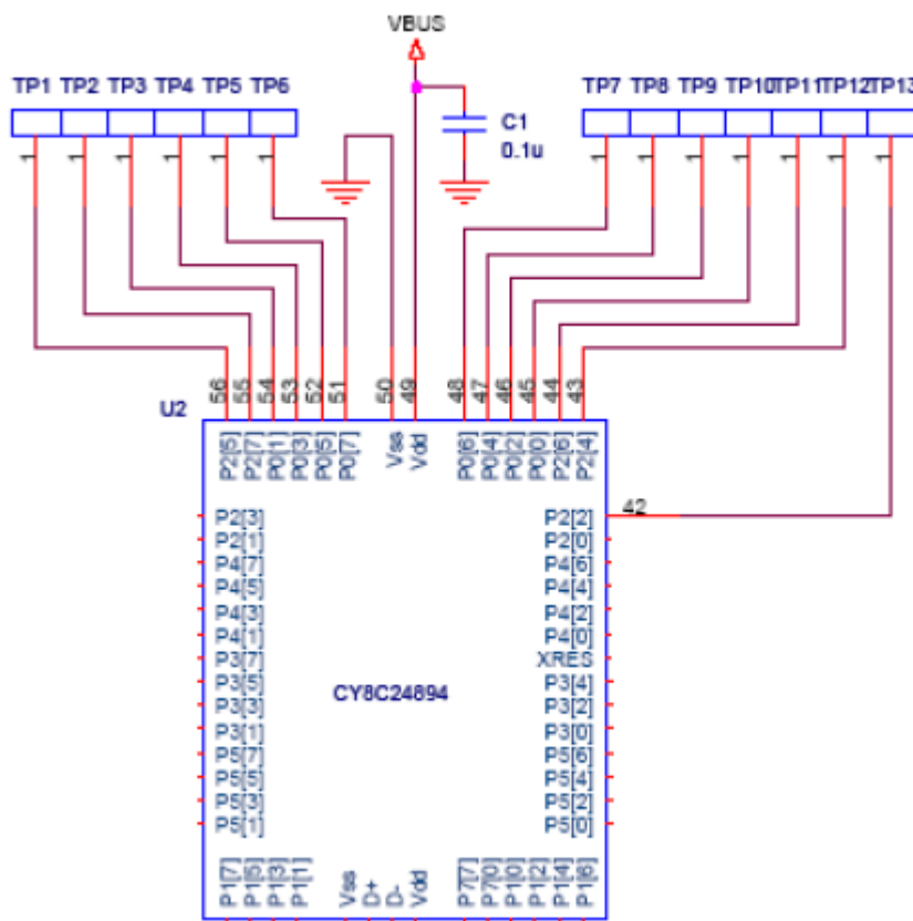
Figure 4-7. GPIO Pin Schematic
