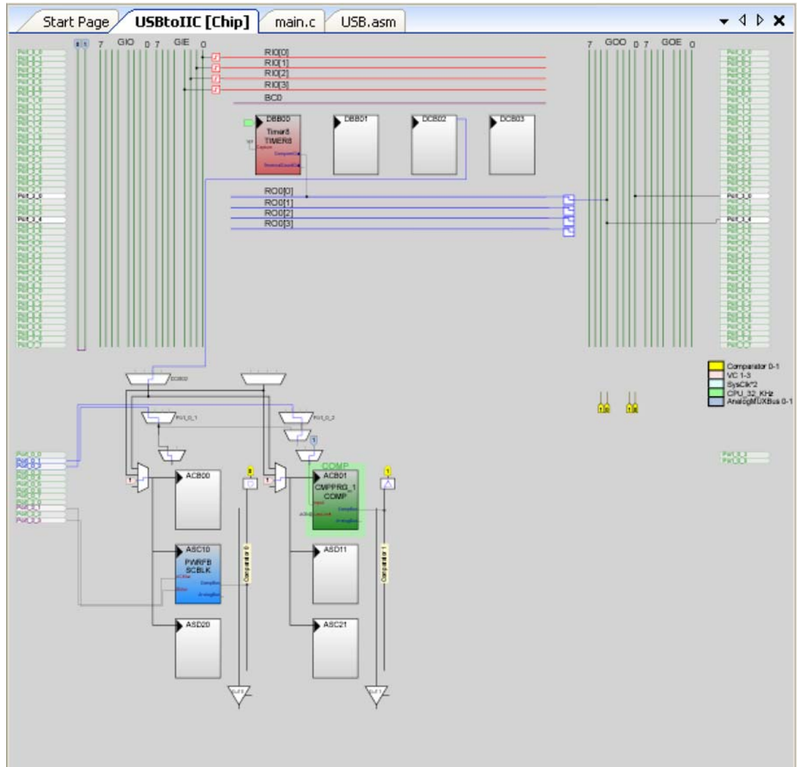
Figure 5-3. Functional Blocks
