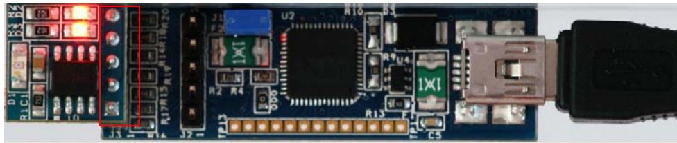
Figure 3-5. Demonstration Board and Bridge Connection
