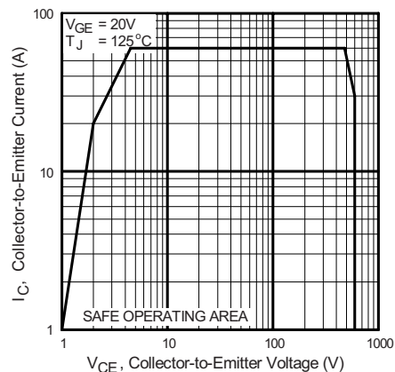
Fig. 12 - Turn-Off SOA
