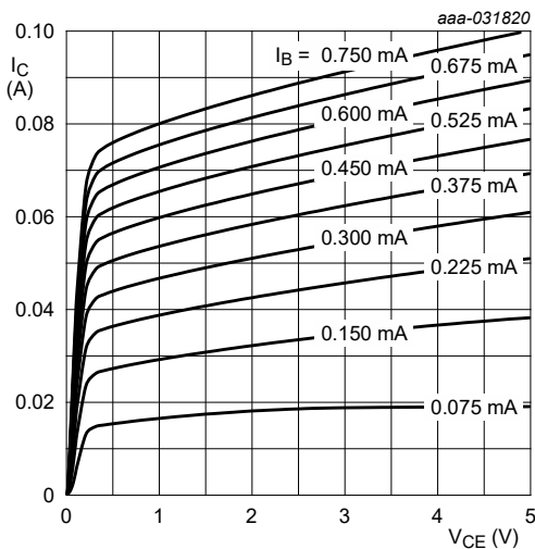
Fig. 11. NHDTC143ZT: Collector current as a function of collector-emitter voltage; typical values
