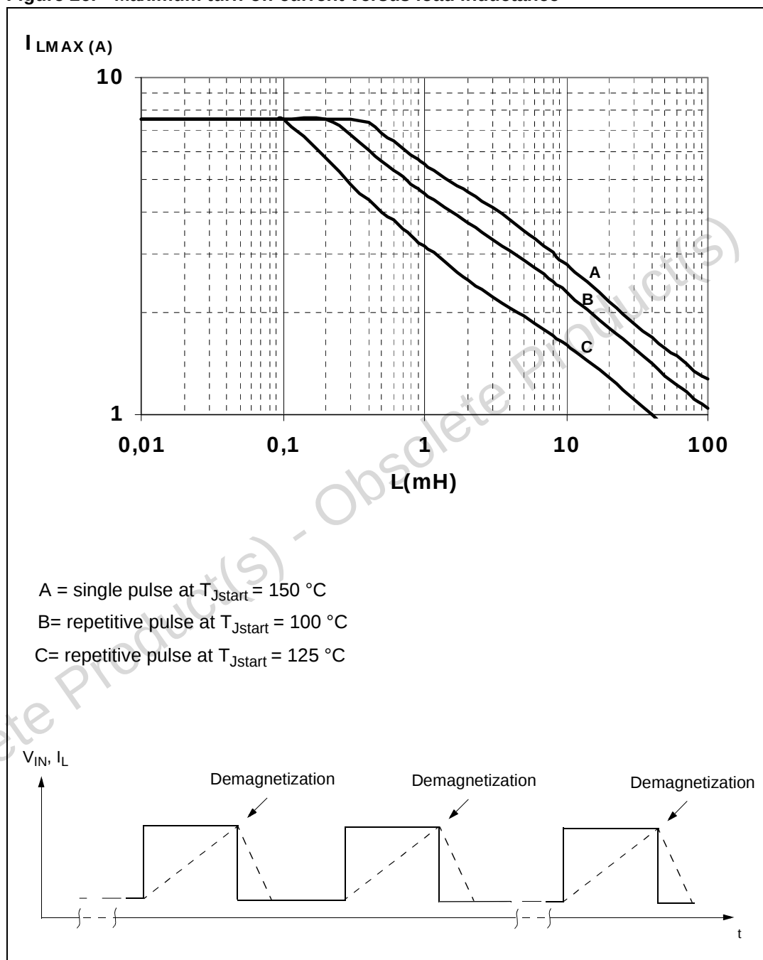
Figure 26. Maximum turn-off current versus load inductance (1)
