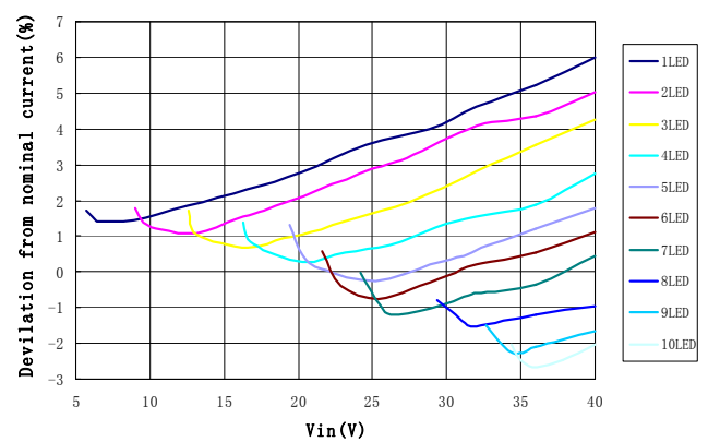
Output current variation with Supply Voltage L=47\mu\text{H} , R_s=0.33\Omega
