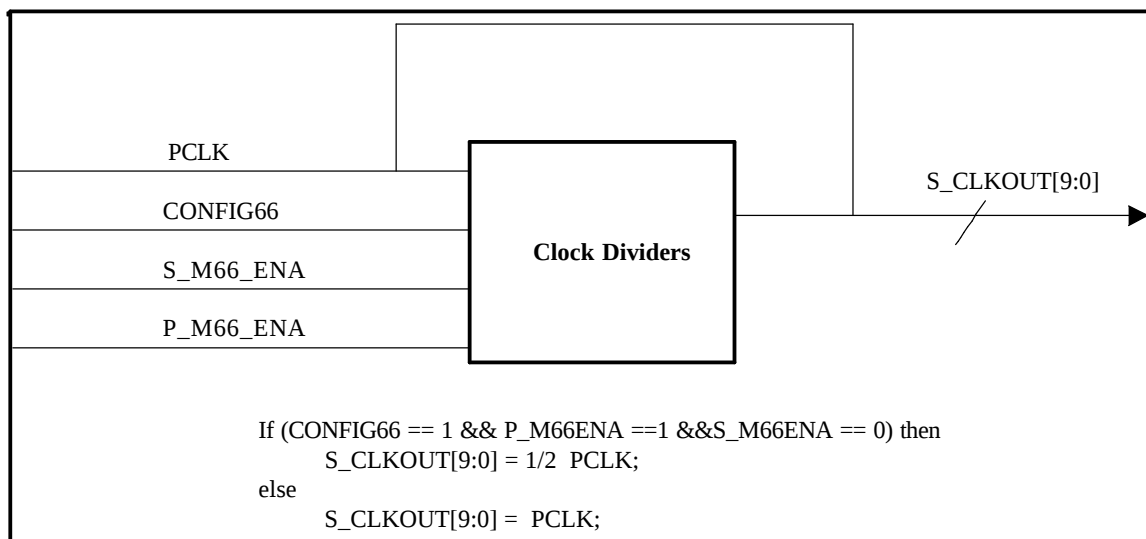
Figure 1. Clock Divider
